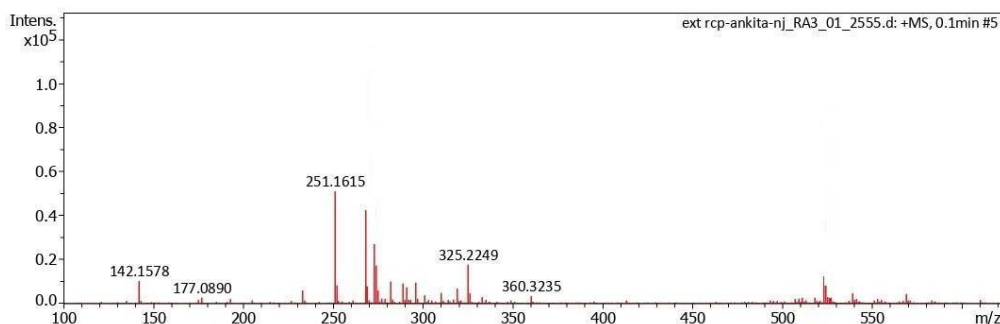
Figure 6: Mass spectra of the isolated compound (Fraction H) of Nardostachys jatamansi Hydro alcoholic extract
