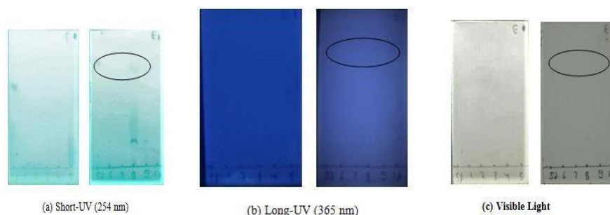
Figure 2: TLC estimation by UV lamp for NJ fractions after column chromatography with std. Std. Sesquiterpenoid. a) Short-UV (254 nm), b) Long-UV (365 nm), c) visible light.
