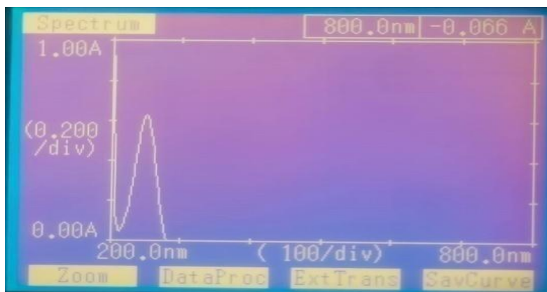
Figure 3: Active constitutes estimation by UV- Spectra of H fraction of Nardostachys jatamansi Hydro alcoholic extract after column chromatography
