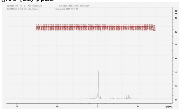
Figure 5: ^1\text{H} -NMR spectra of the isolated compound (Fraction H) of Nardostachys jatamansi Hydro alcoholic extract
