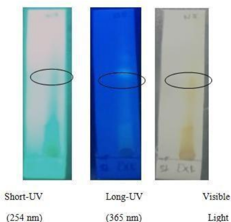
Figure 1: TLC estimation by UV lamp for TLC of NJ with Std. Sesquiterpenoid (Std. = Standard, NJ = Nardostachys Jatamansi )
