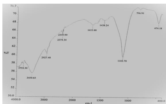
Figure 4: IR spectra of the isolated Fraction H of Nardostachys jatamansi Hydro alcoholic extract
